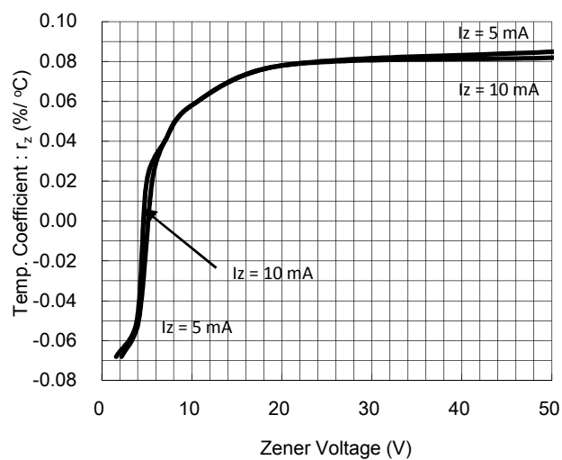
Fig. 3 r_z - V_Z Characteristics
