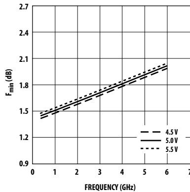
Figure 3. Minimum Noise Figure vs. Frequency and Voltage [1] .
