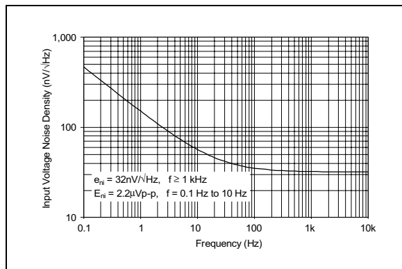
FIGURE 2-26: Input Voltage Noise Density vs. Frequency.
