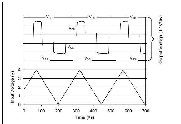
FIGURE 3-1: Maximum Output Voltage Swing.
