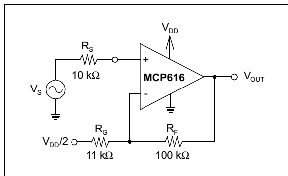
FIGURE 3-10: High gain pre-amplifier for low resistance sources.
