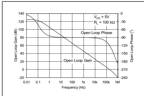
FIGURE 2-25: Open Loop Gain, Phase vs. Frequency.
