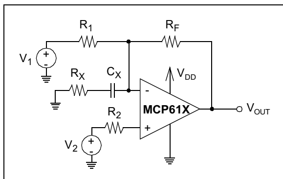
FIGURE 3-6: Circuit for calculating DC Offset.
