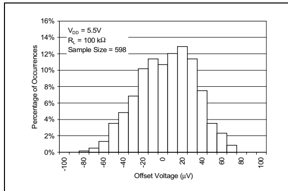
FIGURE 2-1: Histogram of Offset Voltage with V_{DD} = 5.5\text{V} .
