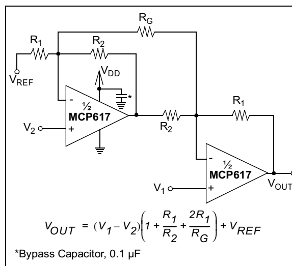
FIGURE 3-11: Two Op Amp Instrumentation Amplifiers.
