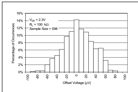
FIGURE 2-2: Histogram of Offset Voltage with V_{DD} = 2.3\text{V} .
