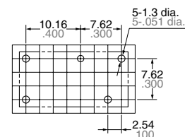
1FormC
