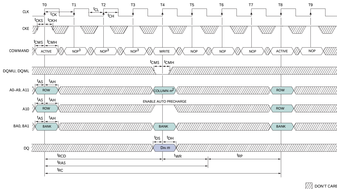
Figure 53: Single Write – With Auto Precharge
