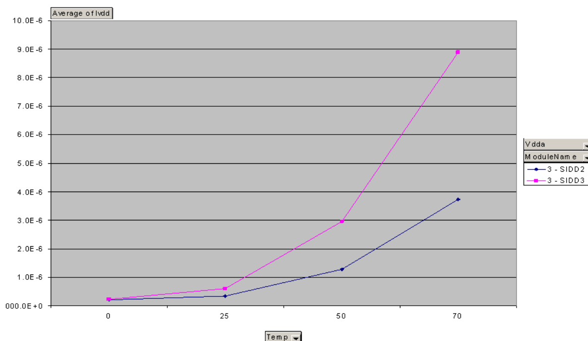
Figure 6. Stop IDD versus Temperature
