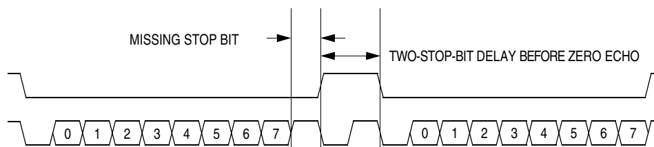
Figure 7-6. Break Transaction
