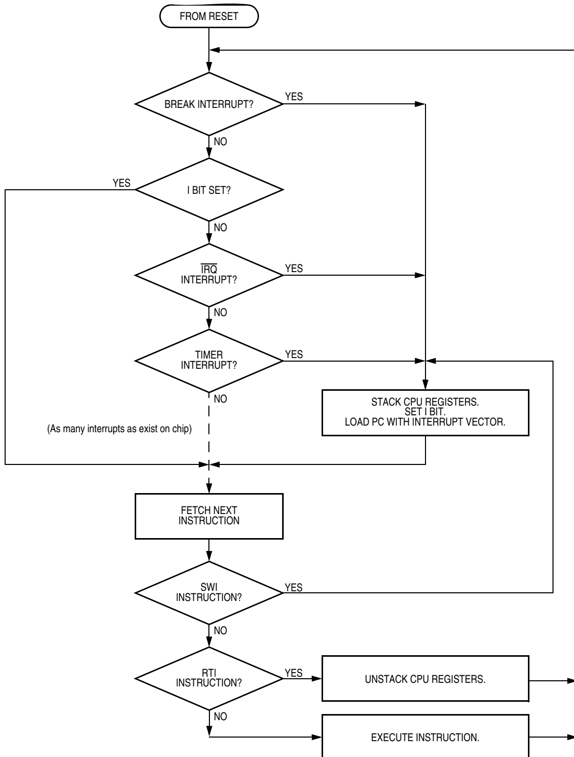
Figure 5-8. Interrupt Processing
