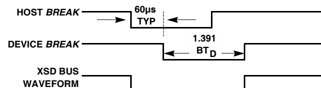
FIGURE 4A. WHEN THE HOST POWER-ON BREAK IS WIDER THAN 60µs
