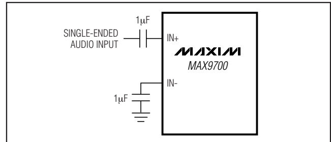
Figure 6. Single-Ended Input
