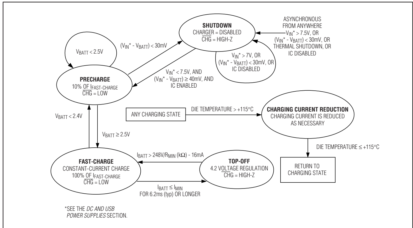
Figure 2. Charge-State Diagram
