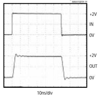
MAX4158/MAX4159 LARGE-SIGNAL PULSE RESPONSE (C L = 20pF)
