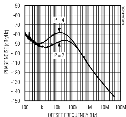
PHASE NOISE
