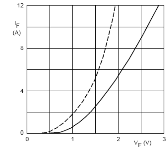
Dotted line: T_j = 175 °C. Solid line: T_j = 25 °C.
