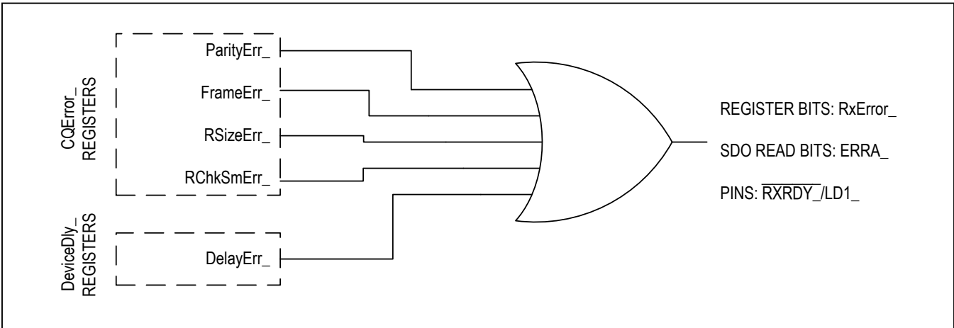
Figure 18. RxError_ Triggers
