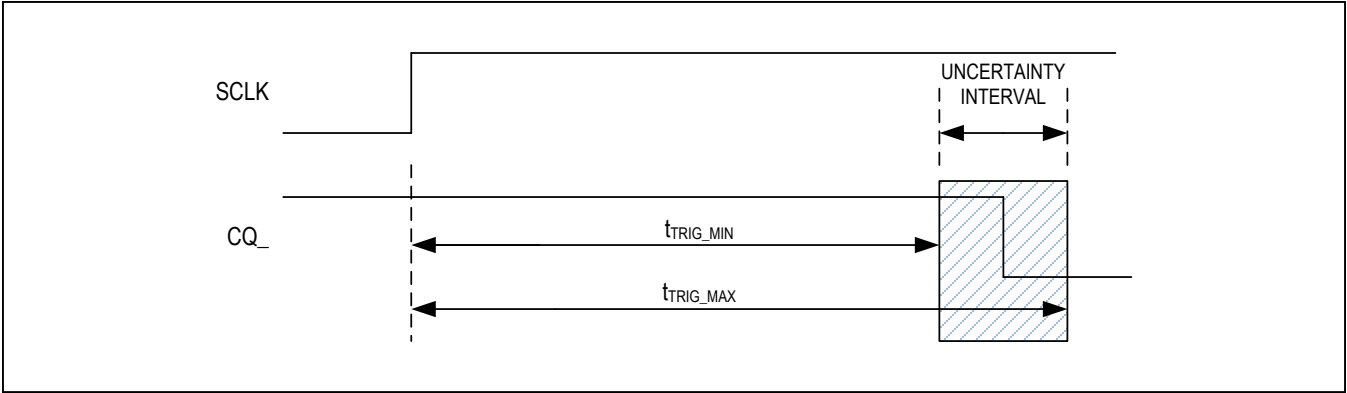
Figure 13. Trigger Delay
