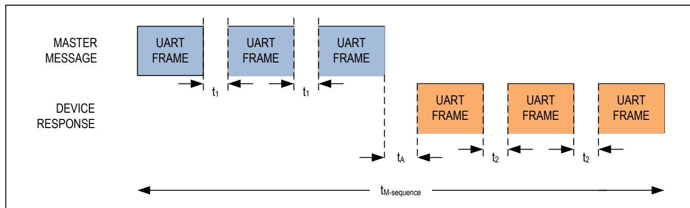
Figure 12. Message Timing
