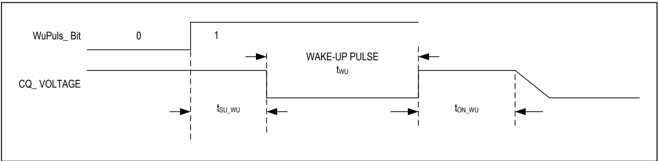
Figure 9. Wake-Up Timing
