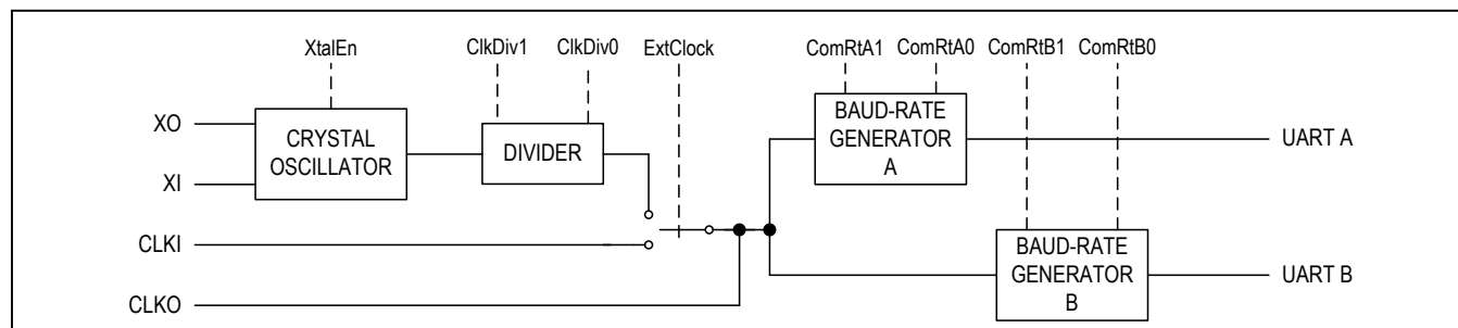
Figure 15. Clock Generation
