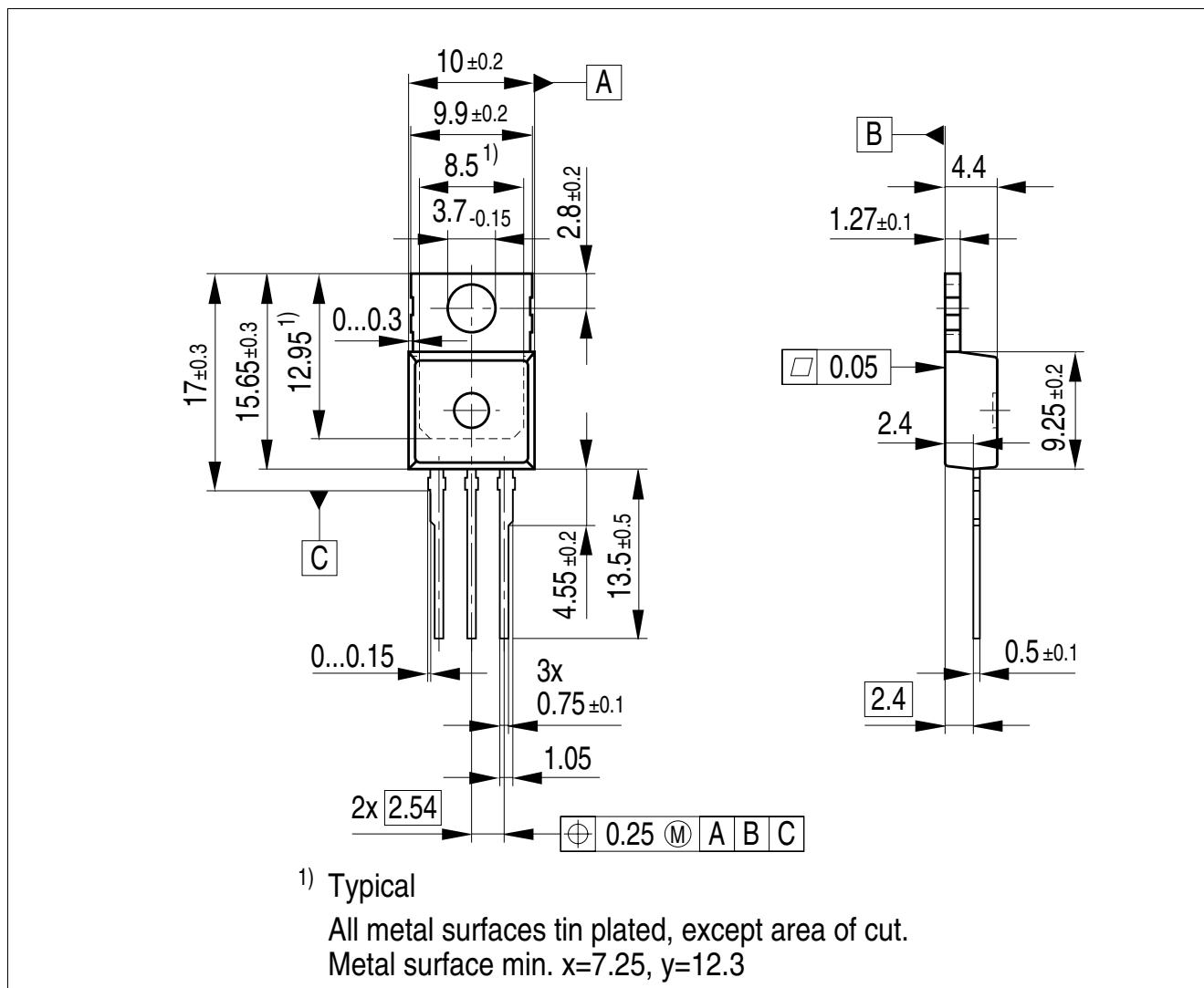
Figure 5 PG-TO220-3
