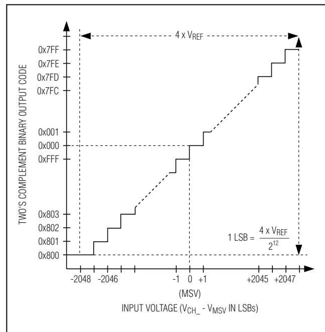
Figure 13. \pm 5V Bipolar Transfer Function
