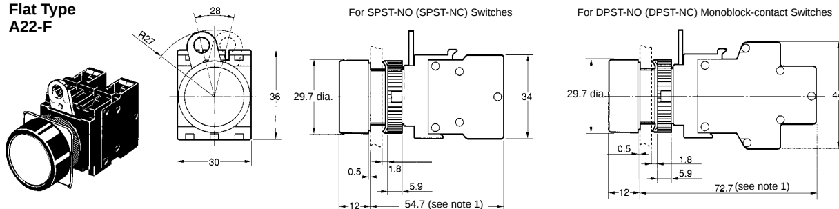
Half-guard Type A22-H, A22L-H
