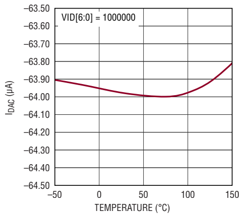
NIDAC vs Temperature
