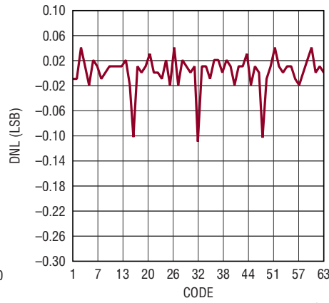
Differential Nonlinearity
