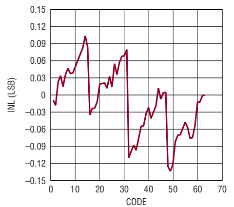
Integral Nonlinearity
