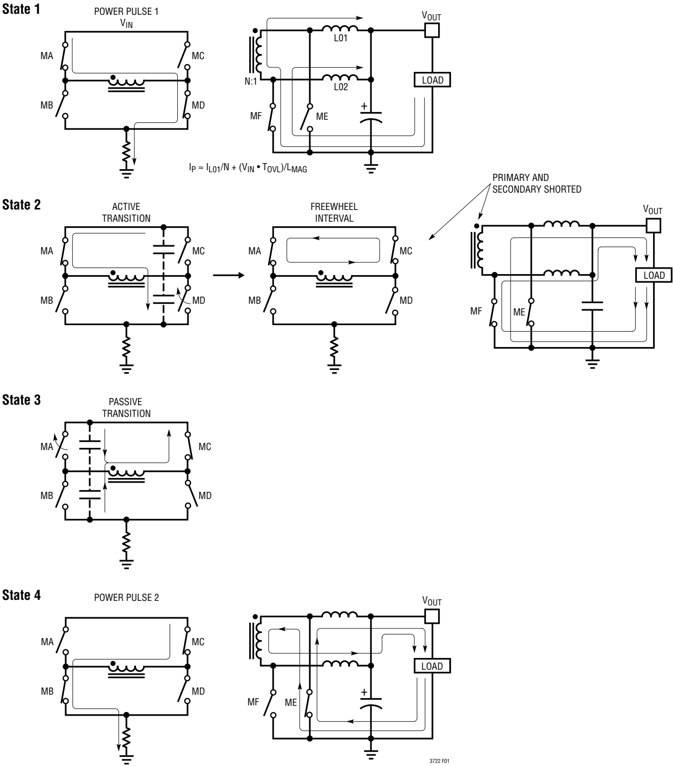
Figure 1. ZVS Operation
