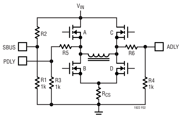
Figure 2. Adaptive Mode
