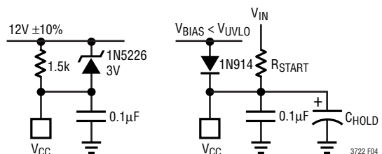
Figure 5. Bias Configurations
