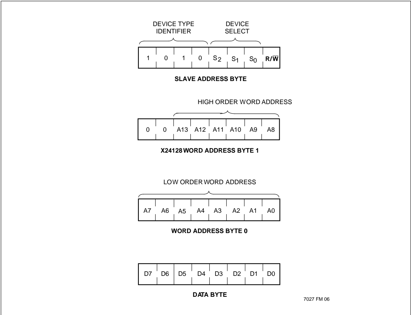
Figure 4. Device Addressing
