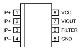
Package LC, 8-Pin SOIC Pin-out Diagram
