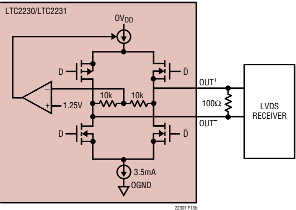
Figure 13b. Digital Output in LVDS Mode
