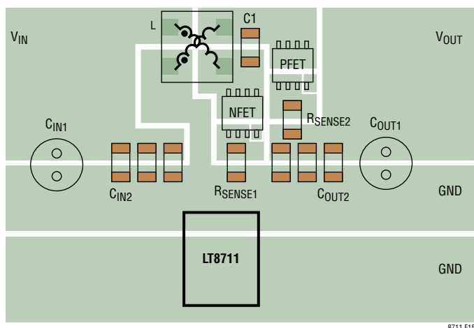
Figure 15. Suggested Component Placement for SEPIC Topology
