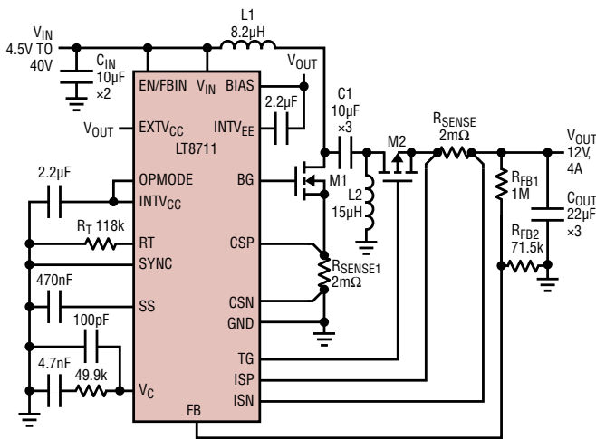
Figure 5. SEPIC Converter—The Component Values Given Are Typical Values for a 200kHz, 4.5V–40V to 12V/4A SEPIC
