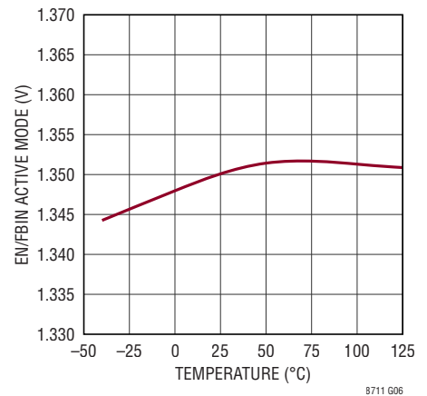
EN/FBIN Active Mode Threshold
