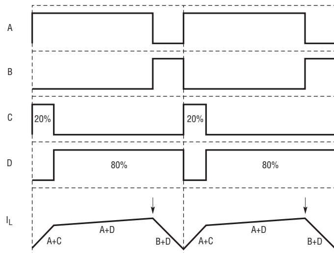
Figure 5. Peak-Buck in Buck-Boost Region ( V_{IN} \sim V_{OUT} )
