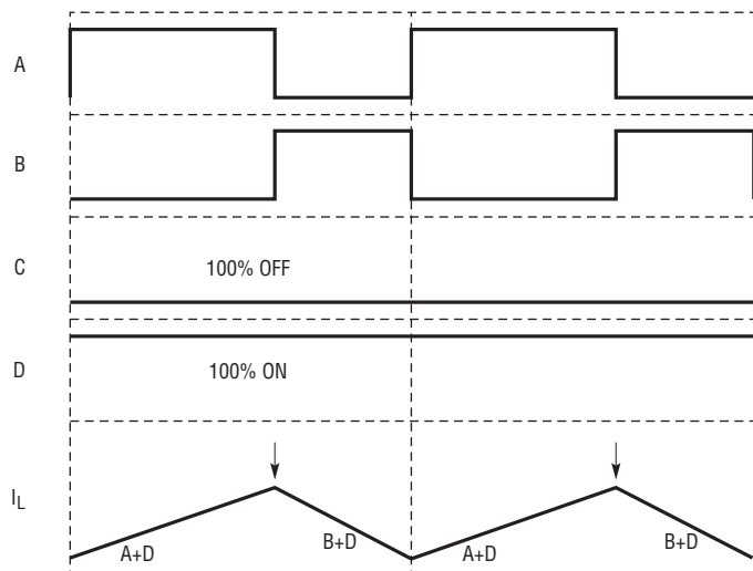
Figure 4. Peak-Buck in Buck Region ( V_{IN} \gg V_{OUT} )
