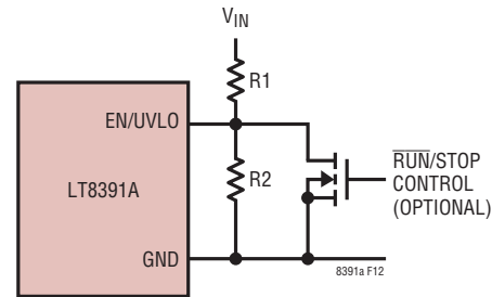
Figure 12. V_{IN} Undervoltage Lockout (UVLO)
