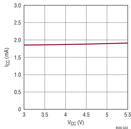
I_{CC} vs V_{CC} , SCKI = 0MHz, SDI = 0MHz, PWMCK = 25MHz
