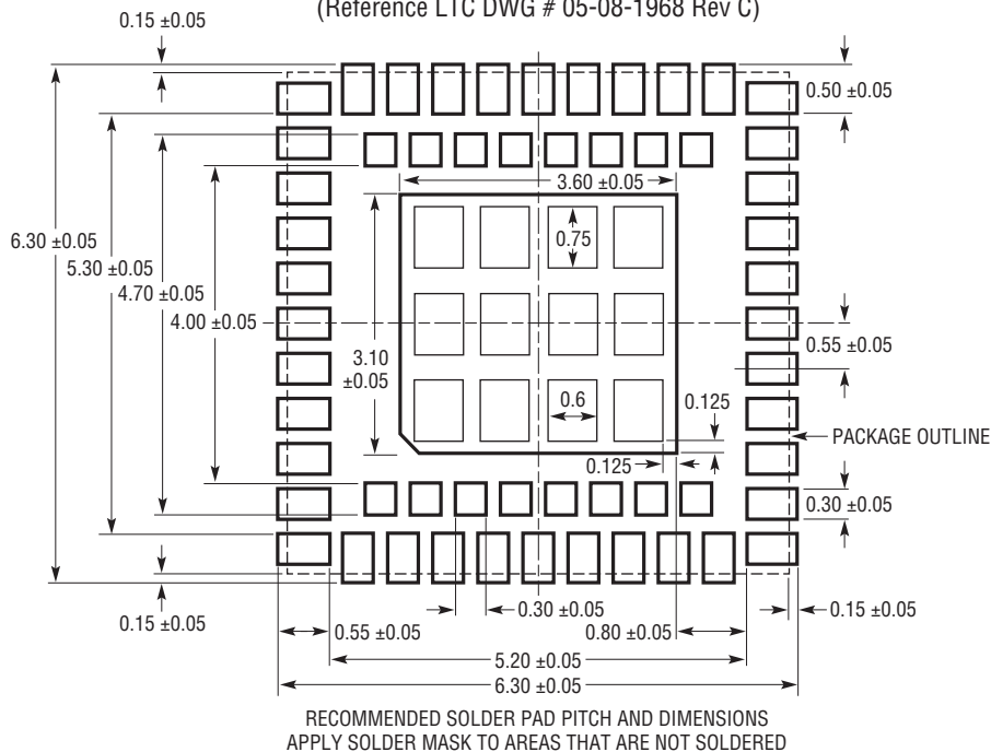
TJ Package 56-Lead Plastic TLA QFN (6mm × 6mm) (Reference LTC DWG # 05-08-1968 Rev C)
