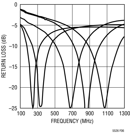
Figure 6. Input Return Loss with Lumped Element Baluns Using Values from Table 2
