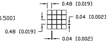
PIXEL DETAIL
