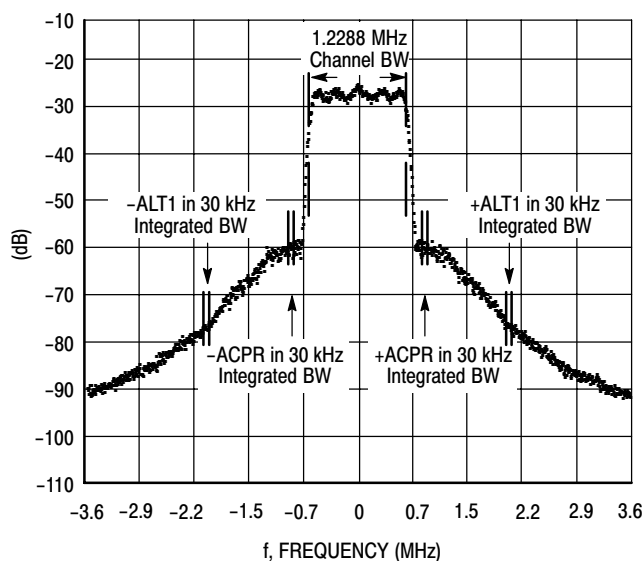
Figure 10. Single-Carrier N-CDMA Spectrum
