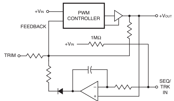
Figure 17. Sequence/Track Simplified Equivalent Schematic
