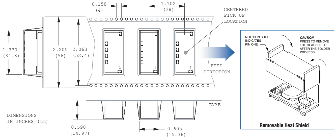
Figure 7. Tape Dimensions
