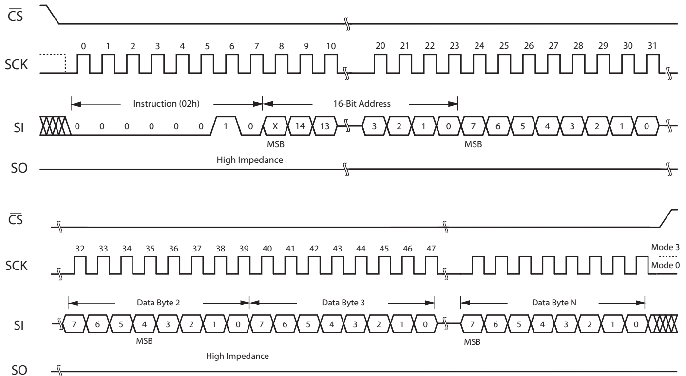
Figure 9 – WRITE
