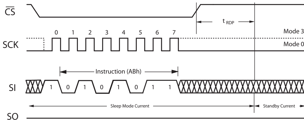
Figure 11 – WAKE
