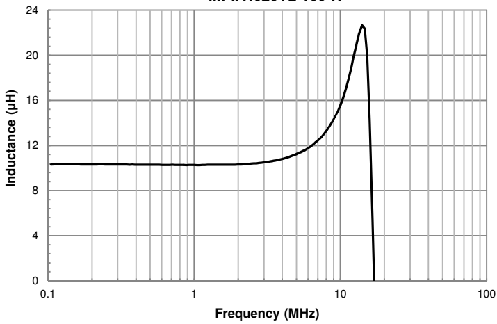
MPIA4020V2-100-R
