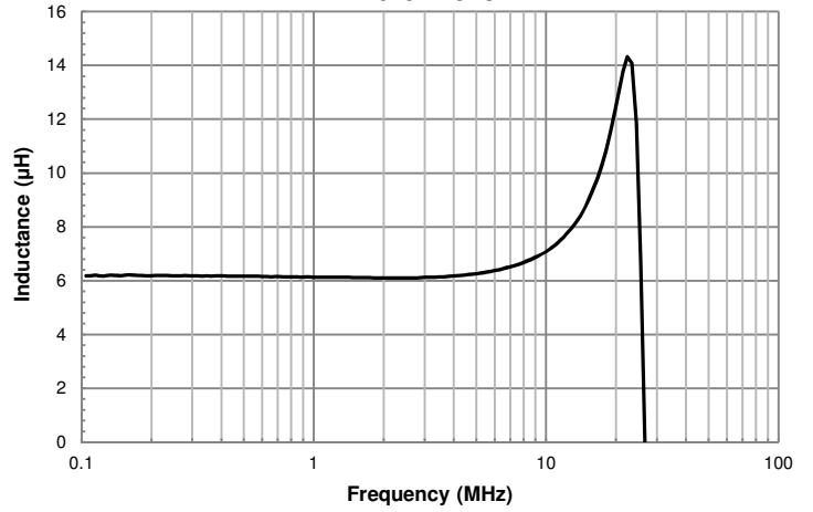
MPIA4020V2-6R8-R
