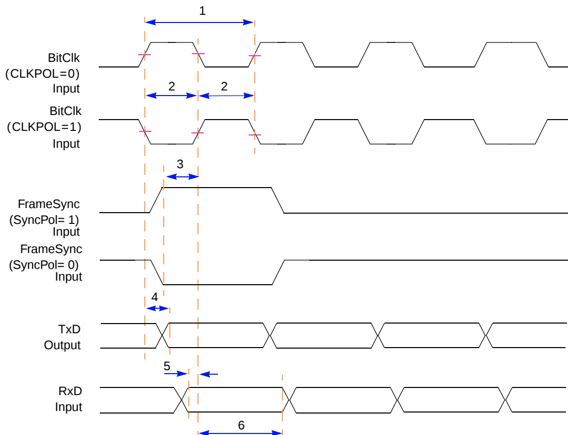
Figure 39. Timing Diagram — 8-,16-, 24-, and 32-bit CODEC/I²S Slave Mode
