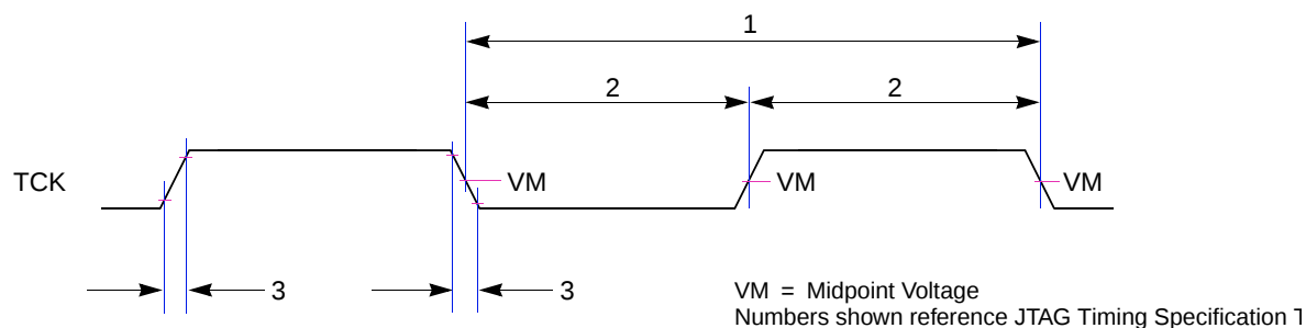
Figure 45. Timing Diagram — JTAG Clock Input
