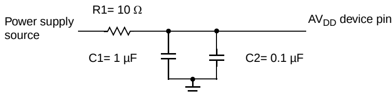
Figure 49. Power Supply Filtering
