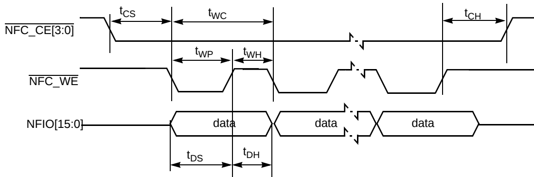
Figure 24. Write Data Latch Timing
