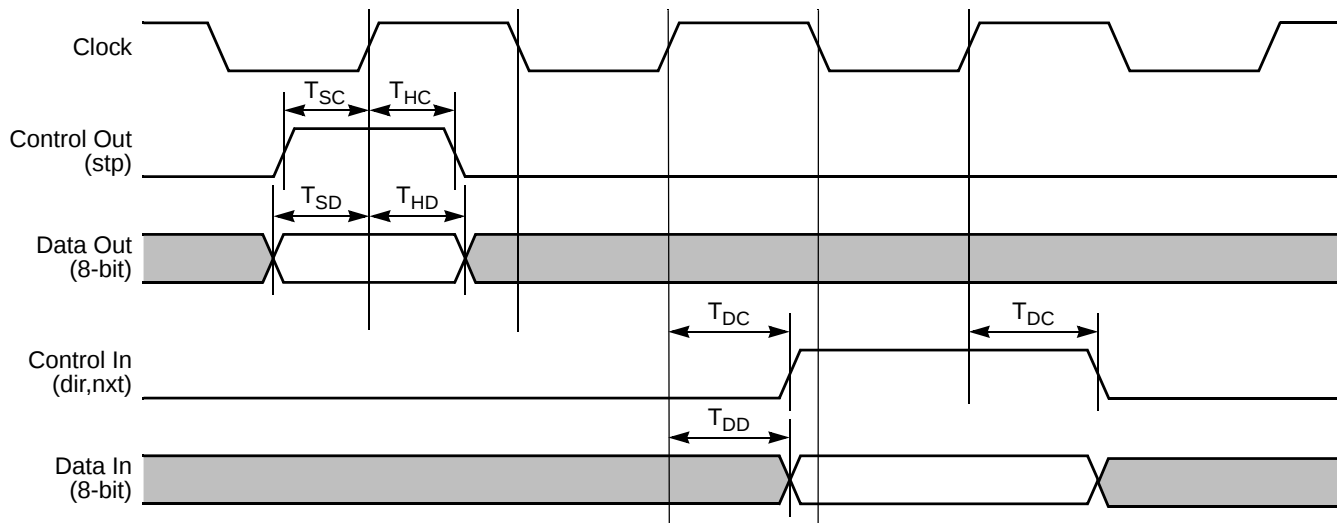
Figure 31. ULPI Timing Diagram
