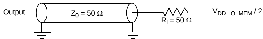
Figure 13. DDR AC Test Load
