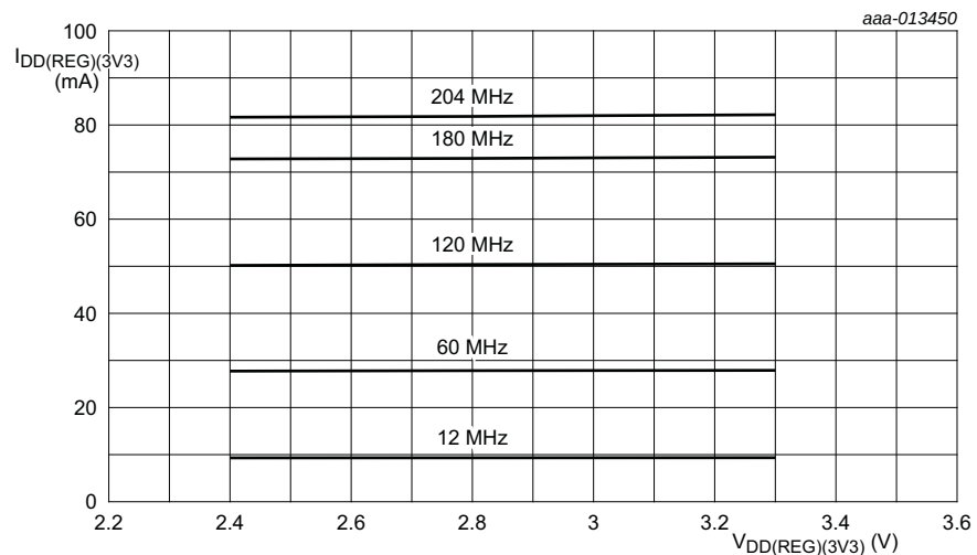
Fig 11. Typical supply current versus regulator supply voltage V_{DD(REG)(3V3)} in active mode
