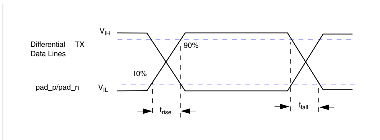
Figure 14. Rise/fall time
