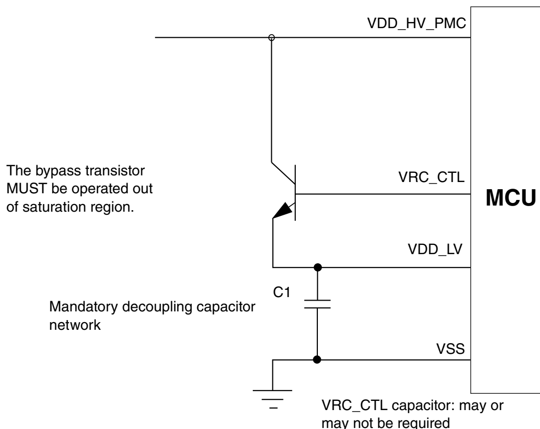
Figure 18. Regulator example
