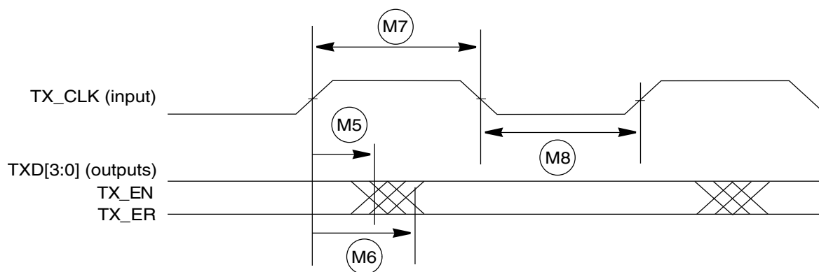
Figure 42. MII-lite transmit signal timing diagram
