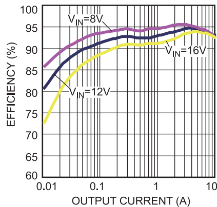
Figure 50 — Efficiency Curve
