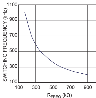
Switching Frequency vs. RFRQE
