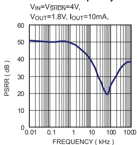
PSRR vs.Frequency
