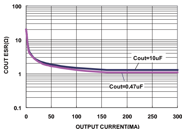
Figure 2—Relationship between ESR and LDO Stability
