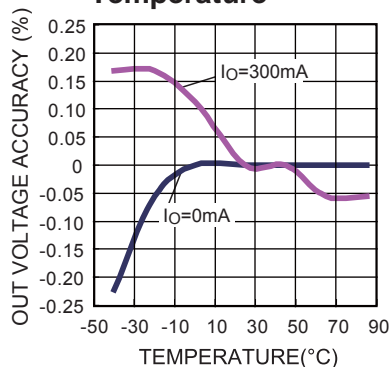
Out1 Voltage Accuracy vs. Temperature
