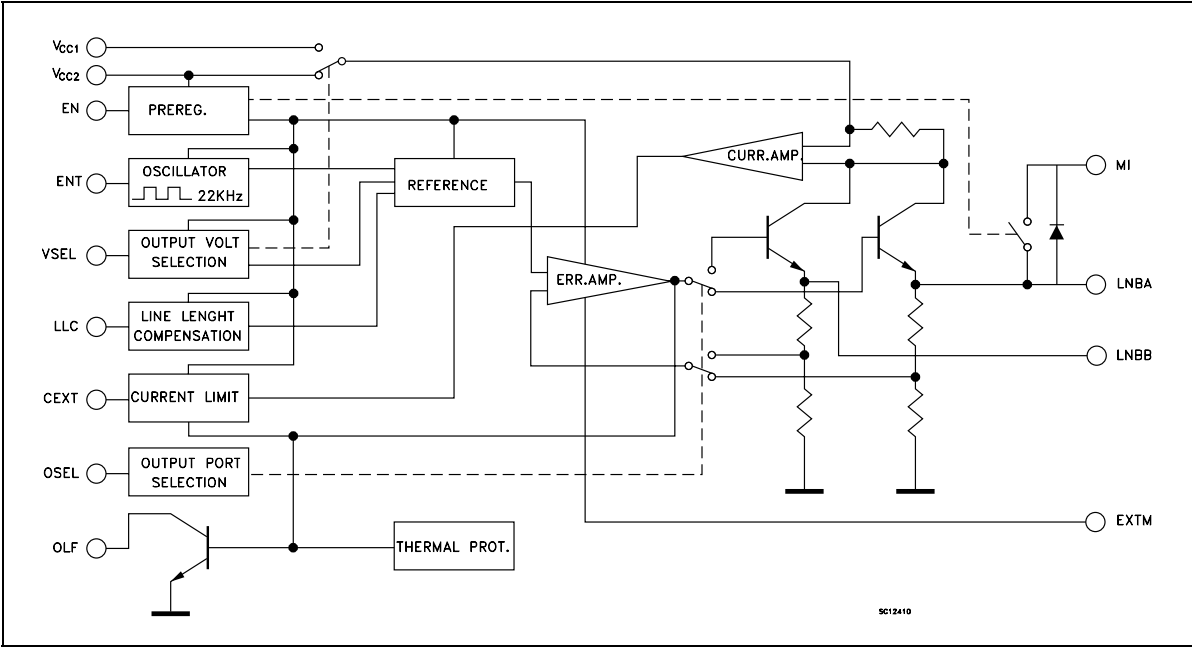
Figure 2. Block diagram
