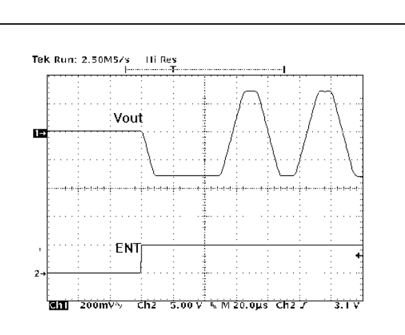
Figure 20. 22KHz Tone
