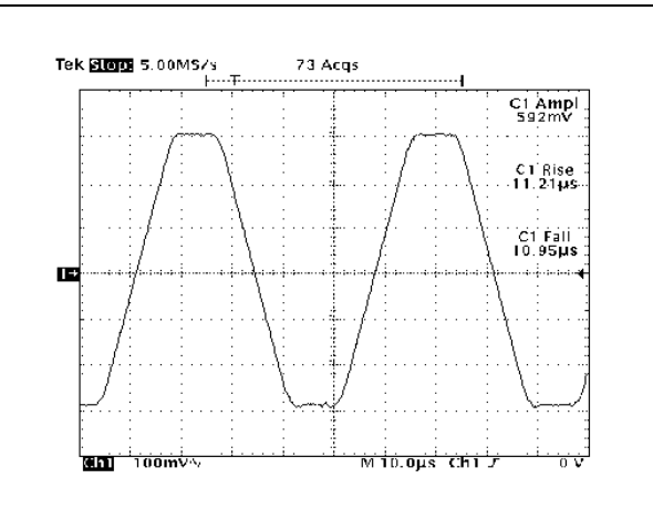
Figure 20. 22KHz Tone
