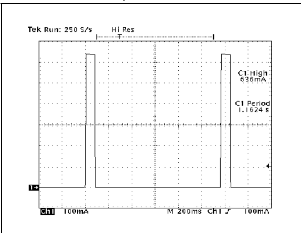
Figure 19. Tone disable
