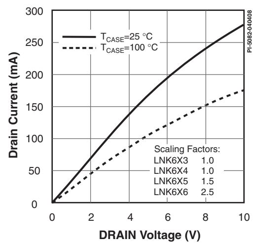
Figure 16. Output Characteristic.
