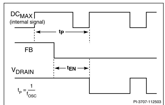
Figure 9. LinkSwitch-TN Output Enable Timing.
