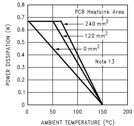
Power Derating Curves for 8 Bump microSMD ( P_{D\text{MAX}} = 670\text{mW} )
