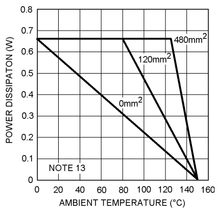
Power Derating - 10 Pin LD Pkg P_{D\text{MAX}} = 670\text{mW} , 5V, 8Ω
