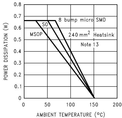
Power Derating Curves (P_{D\text{MAX}} = 670\text{mW})
