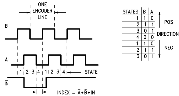
FIGURE 9. Quadrature Encoder Signals
