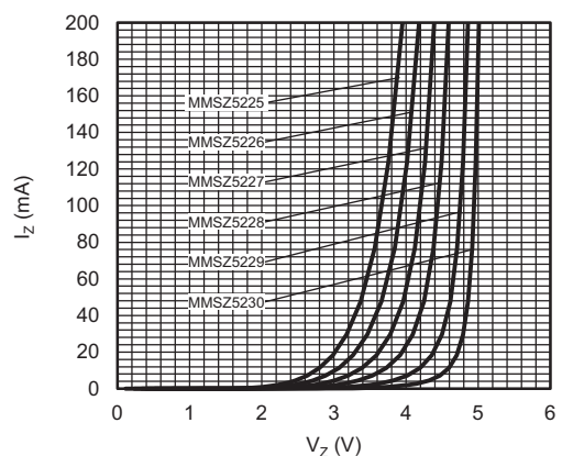
Fig. 6 - Breakdown Characteristics
