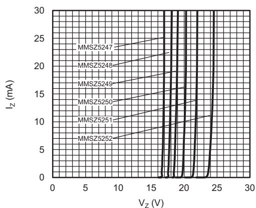
Fig. 3 - Breakdown Characteristics
