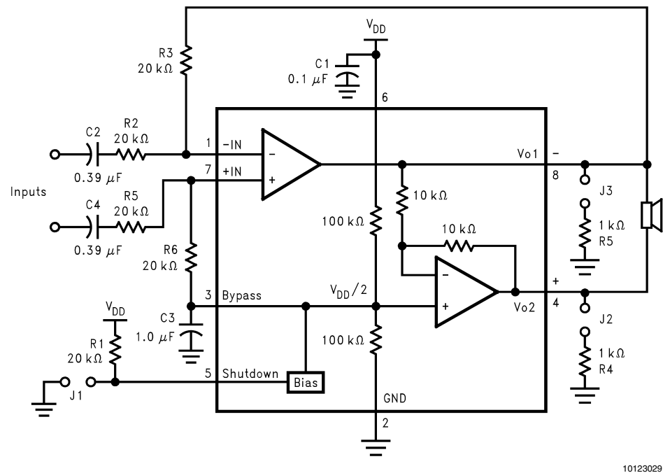
FIGURE 3. Differential Amplifier Configuration for LM4872
