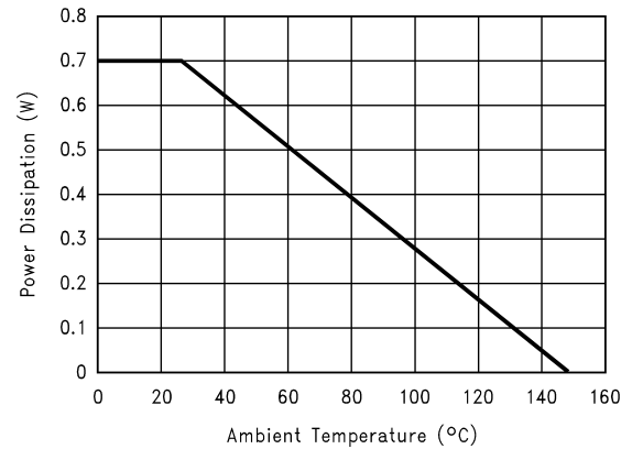
LM4900MM Power Derating Curve
