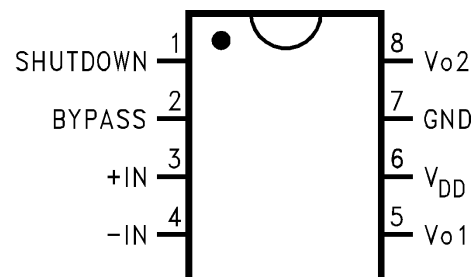
Connection Diagram
