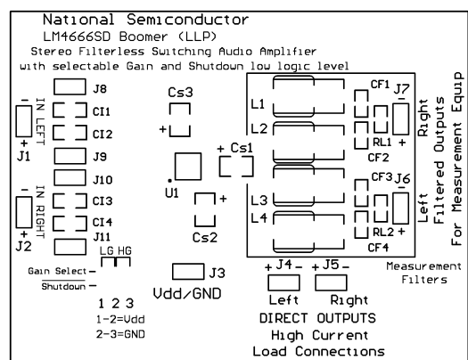
Silk Screen
