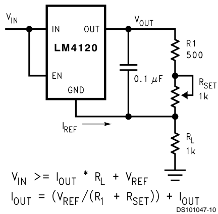
Programmable Current Source
