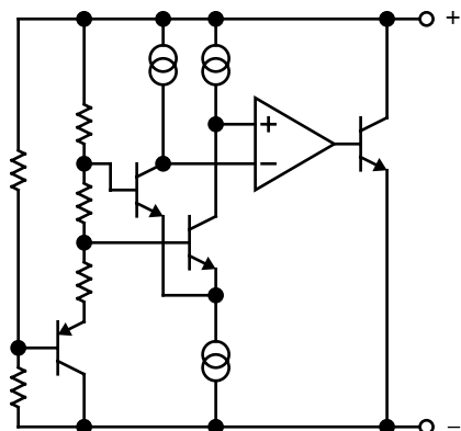
Functional Diagram LM4040, LM4041 Fixed
