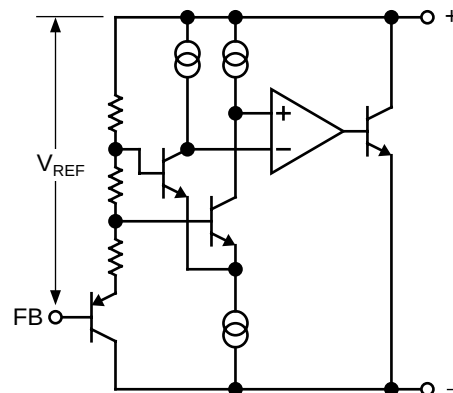
Functional Diagram LM4041 Adjustable
