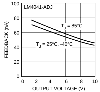
Feedback Current vs. Output Voltage and Temperature
