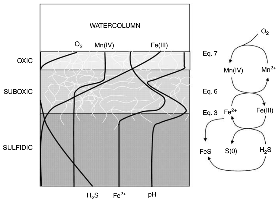
Figure 9 Overview of the main geochemical reactions in the oxic (dashed), suboxic (light gray) and sulfidic (dark gray) zones, and the schematic porewater profiles. The profiles are not quantitative. The distribution of Beggiatoa is indicated by the white filaments.
